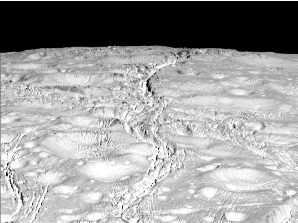
This closeup view of the north pole of Saturn's moon Enceladus shows thin cracks crisscrossing through the ice. The photo was taken at a distance of 4,000 miles from Enceladus. Photo credit: NASA/JPL-Caltech/Space Science Institute
