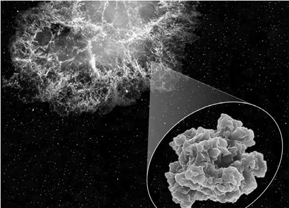
An electron microscope image of a micron-sized supernova silicon carbide, SiC, stardust grain (lower right) extracted from a primitive meteorite. Photo credit: Carnegiescience.edu
